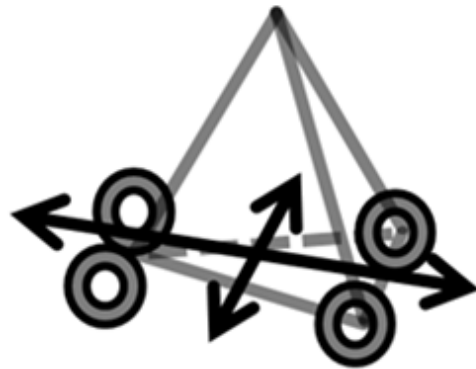
Stability tetrahedron
